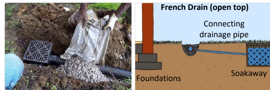
Construction of a French/Filter Drain (left) and combining a French drain with a soakaway storage can help to minimise flooding around your property provided that the ground conditions are suitable (right)
