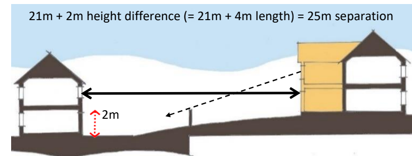
Where there is a change in levels, the separation distance between an extension and an opposing window may need to be increased to maintain adequate levels of privacy
