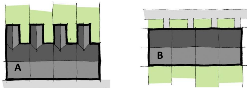
Plan of traditional terraces (A) with projecting rear wings and modern terraces with 'flat back' (B)
